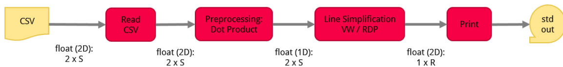
Figure 4.3: Line simplification pipeline for single file (pipeline P4.1)
